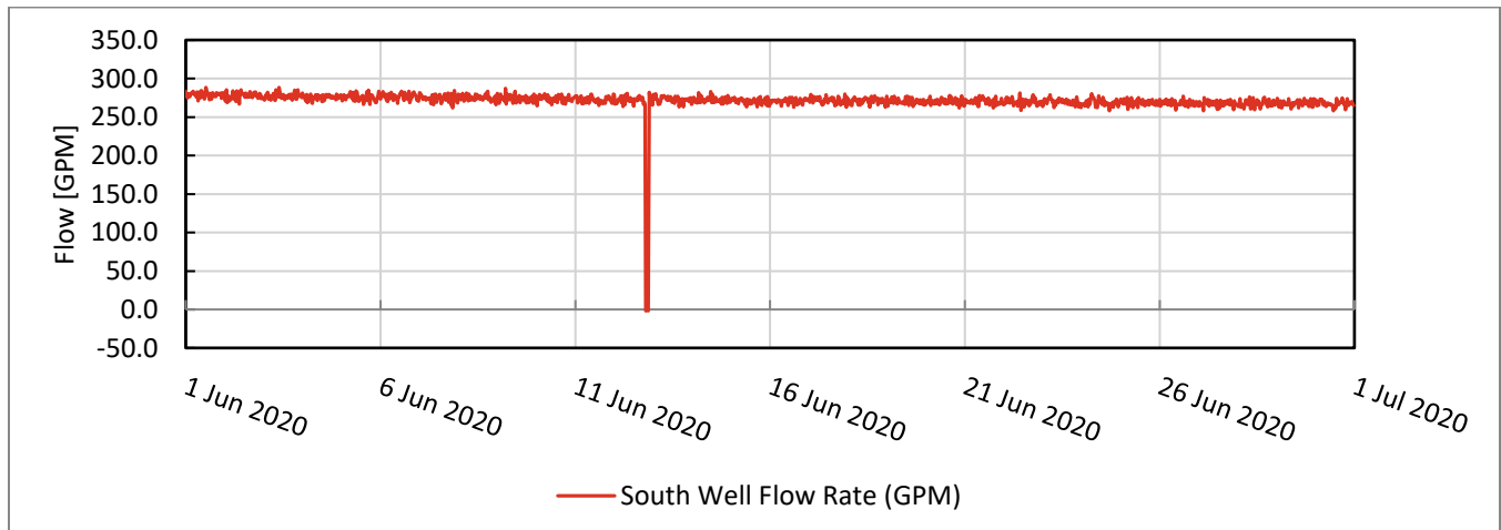
Figure 2 – South Well Production Rate (June 2020)
